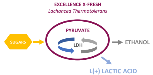
Figure 1: Simplified Metabolism of Lachancea Thermotolerans
